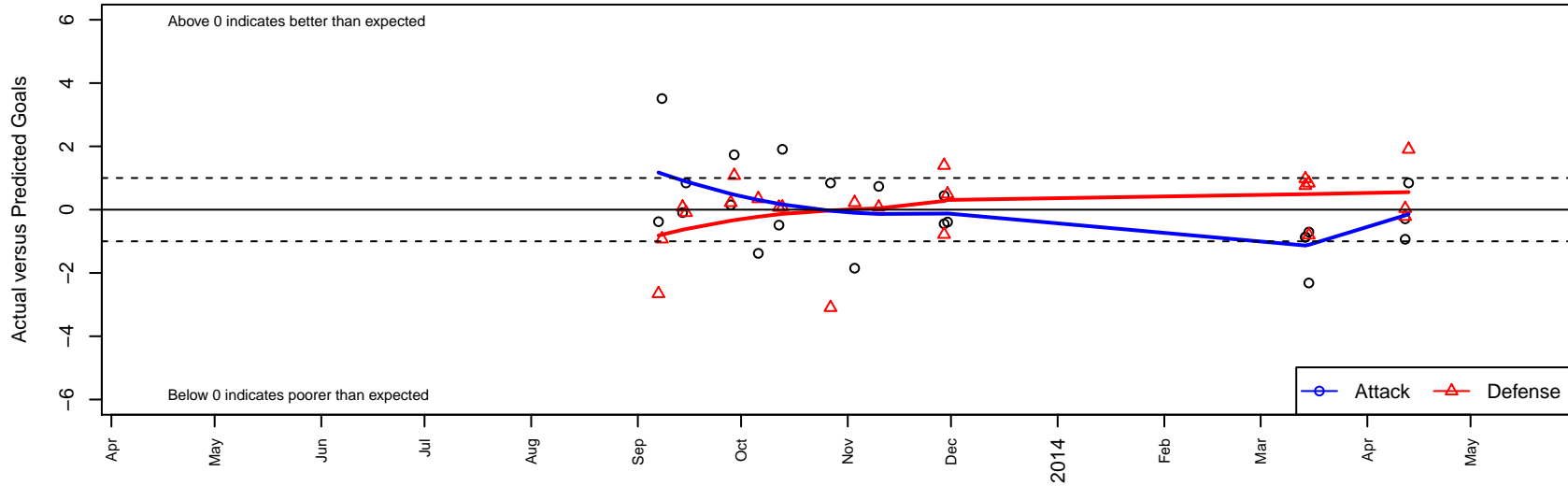
IE Surf B96 Dots are actual minus expected GF (blue circles) and GA (red triangles). Blue line is smoothed change in attack strength. Red is smoothed change in defense strength.
